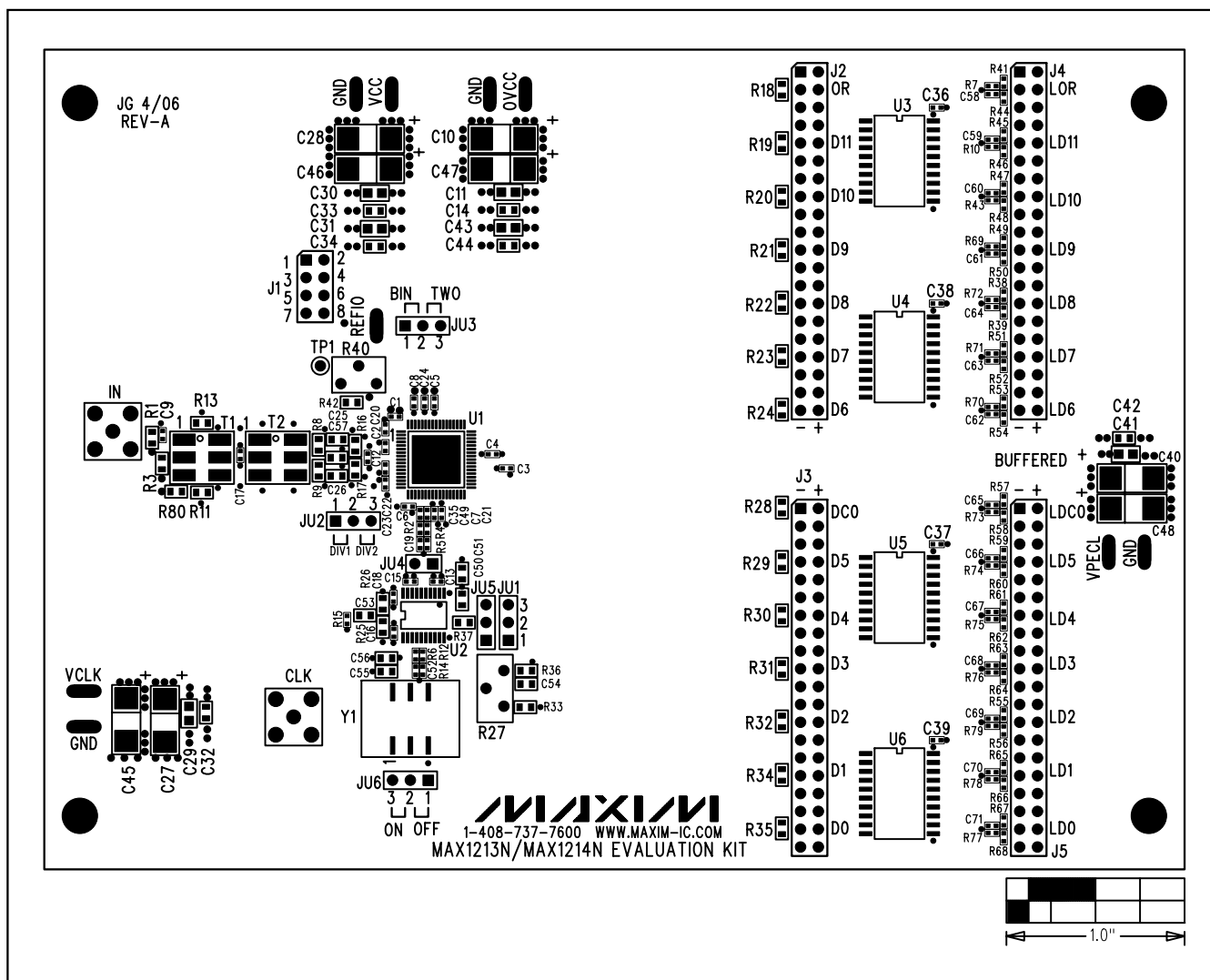
Figure 2. MAX1213N/MAX1214N EV Kit Component Placement Guide—Component Side
